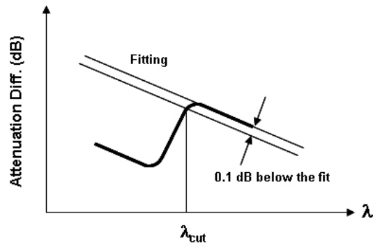
Figure 5: Plot for Cut-off Wavelength Measurement
