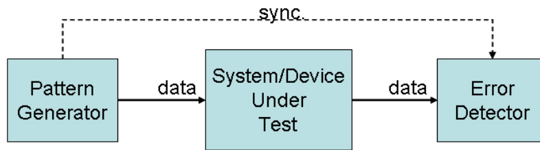
Figure 10: General BER Test Set-up
