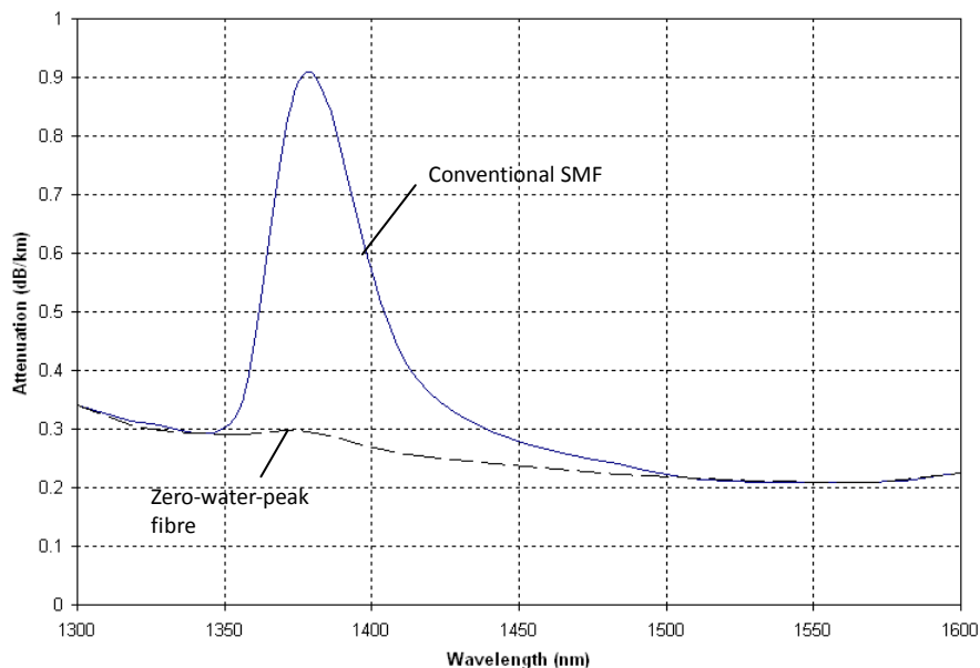
Figure 8: Attenuation Losses for a Single-mode Fibre
