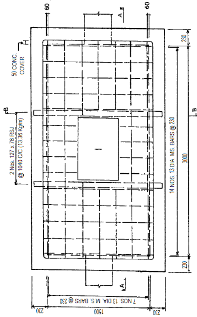
FIGURE 11.31: MANHOLE DRAWINGS - TYPE MX5 (DRAWING 1 OF 3)
