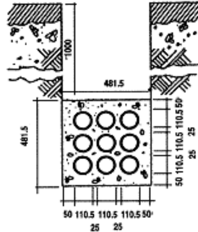
SECTION 9 way pipe formation DRAWING NO 1e
