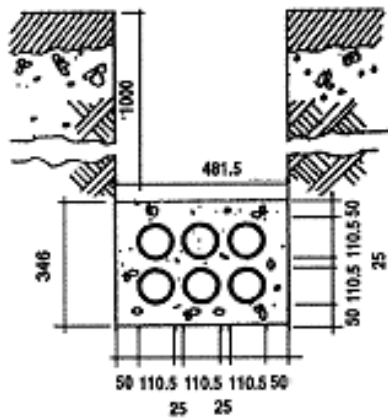
SECTION 6 way pipe formation DRAWING NO 1d
