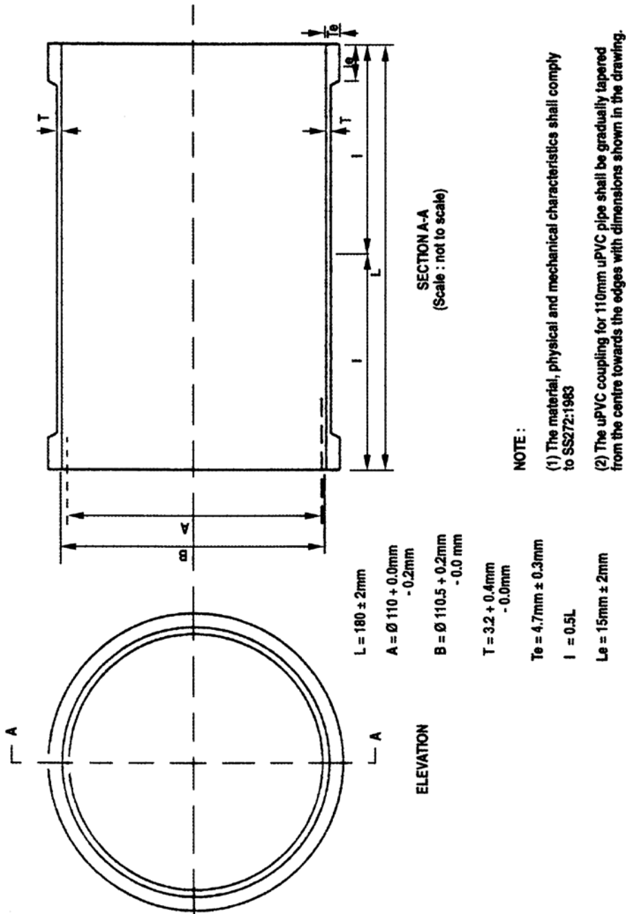
FIGURE 11.1: INJECTION MOULDED UPVC COUPLING FOR 110MM NOMINAL SIZE UPVC PIPE
