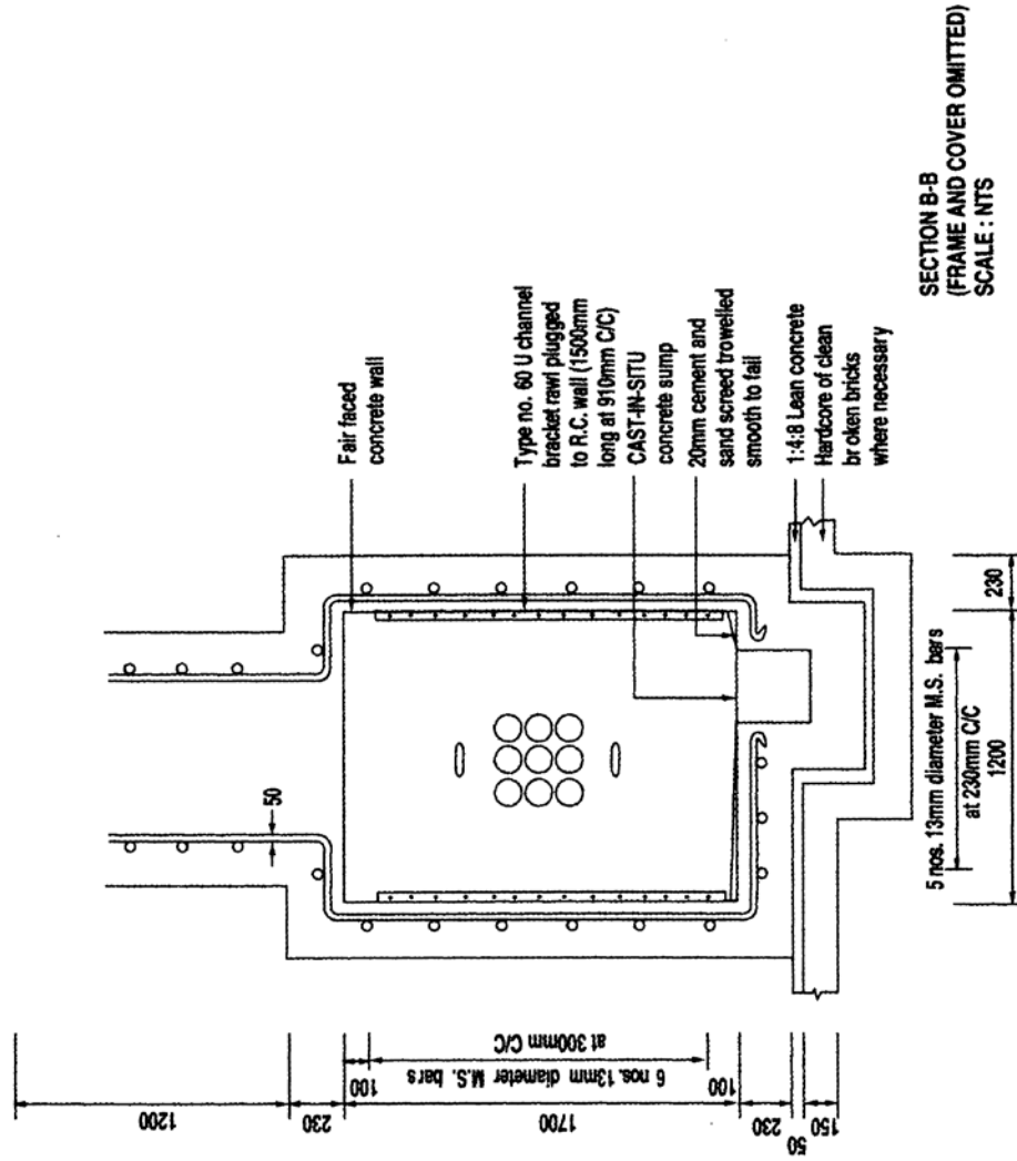
FIGURE 11.21: MANHOLE DRAWINGS - TYPE MX3
