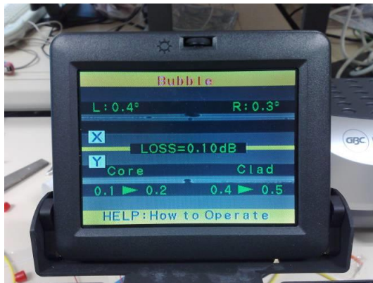
Figure 38: The Fusion Splicer Estimates the Splice Loss (Courtesy of Fujikura Ltd)
