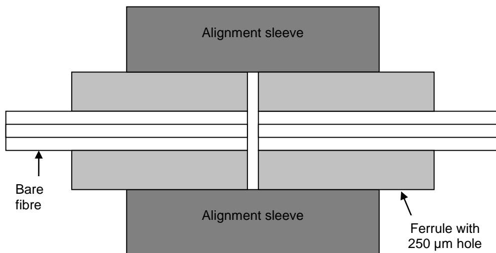
Figure 2: An Alignment Sleeve is used in the Mating Adapter to Aid Ferrule Alignment
