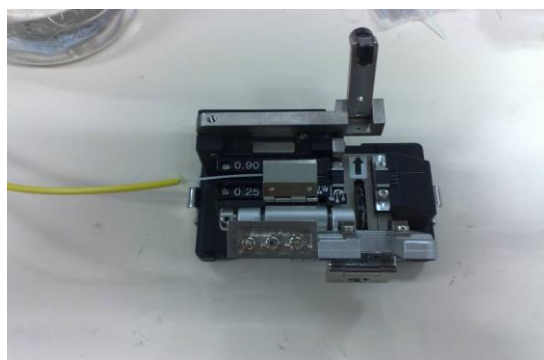
Figure 32: The Bare Fibre is Positioned and Clamped on the Fibre Cleaver before it is Cleaved
