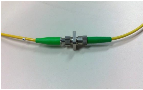
Figure 14: FC/APC Cables Connected via an FC-to-FC Adapter
