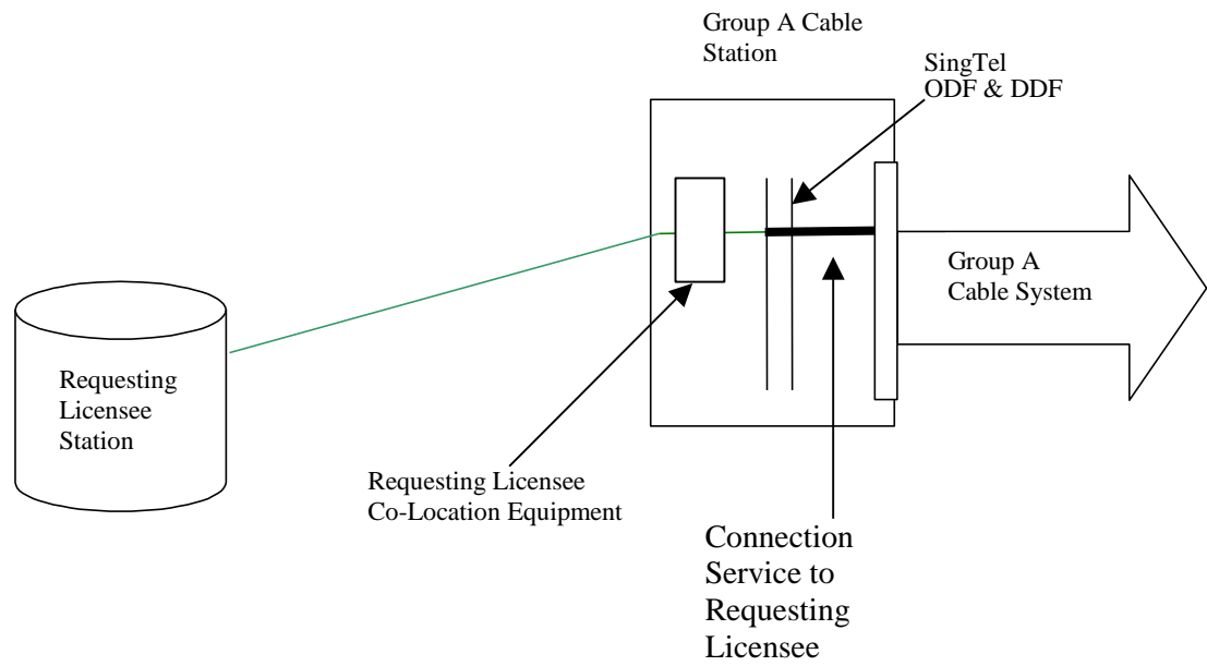
Connection Service diagram for Group A Submarine Cable Systems
