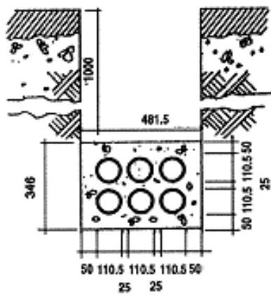
SECTION 6 way pipe formation DRAWING NO 1d
