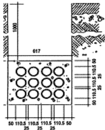
SECTION 12 Way pipe formation DRAWING NO 1f
