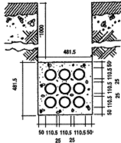
SECTION 9 way pipe formation DRAWING NO 1e
