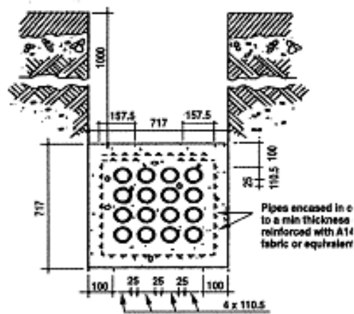
SECTION 16 Way pipe formation DRAWING NO 1g
