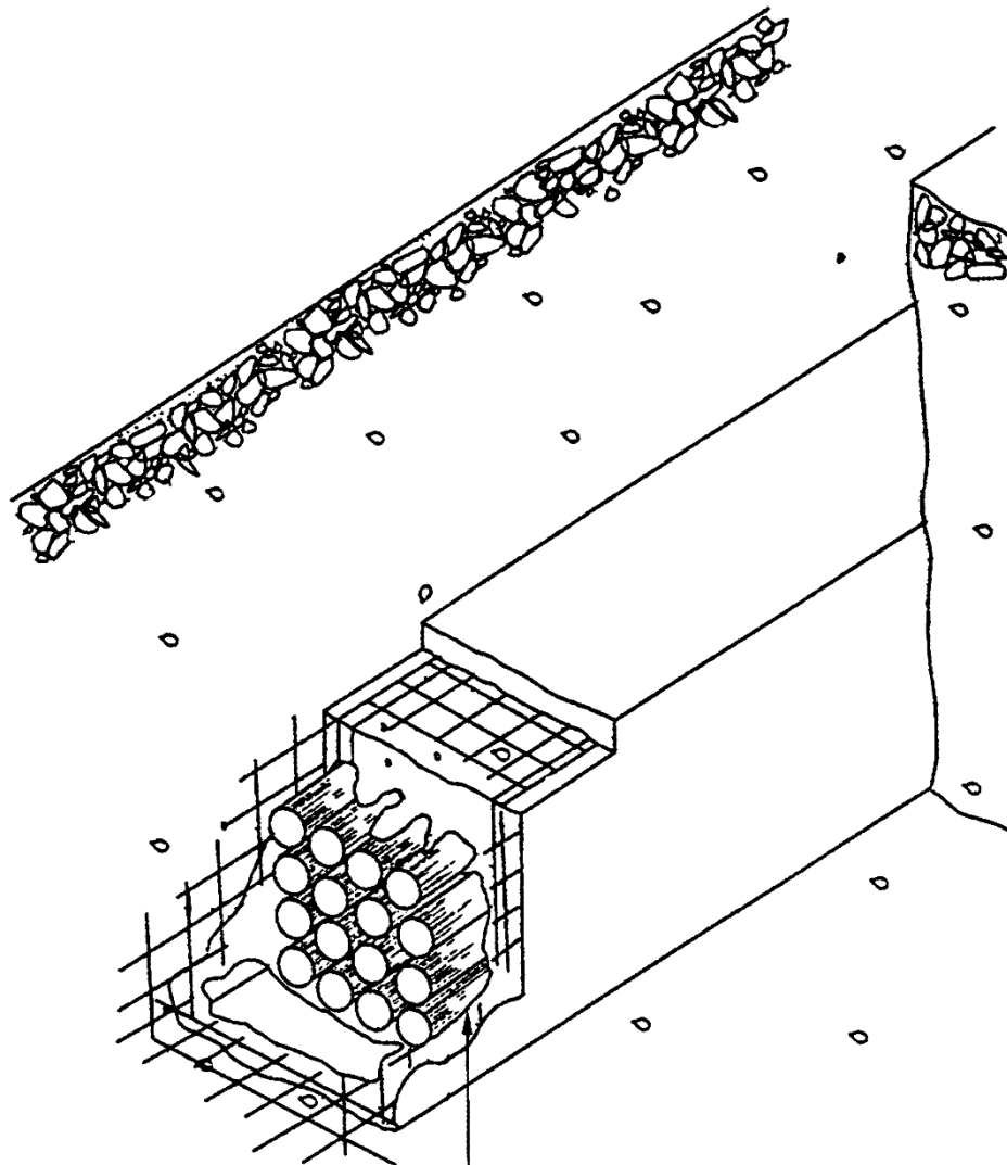
FIGURE 11.34: DRAWINGS OF MULTI-WAY PIPELINES (CONT'D)
