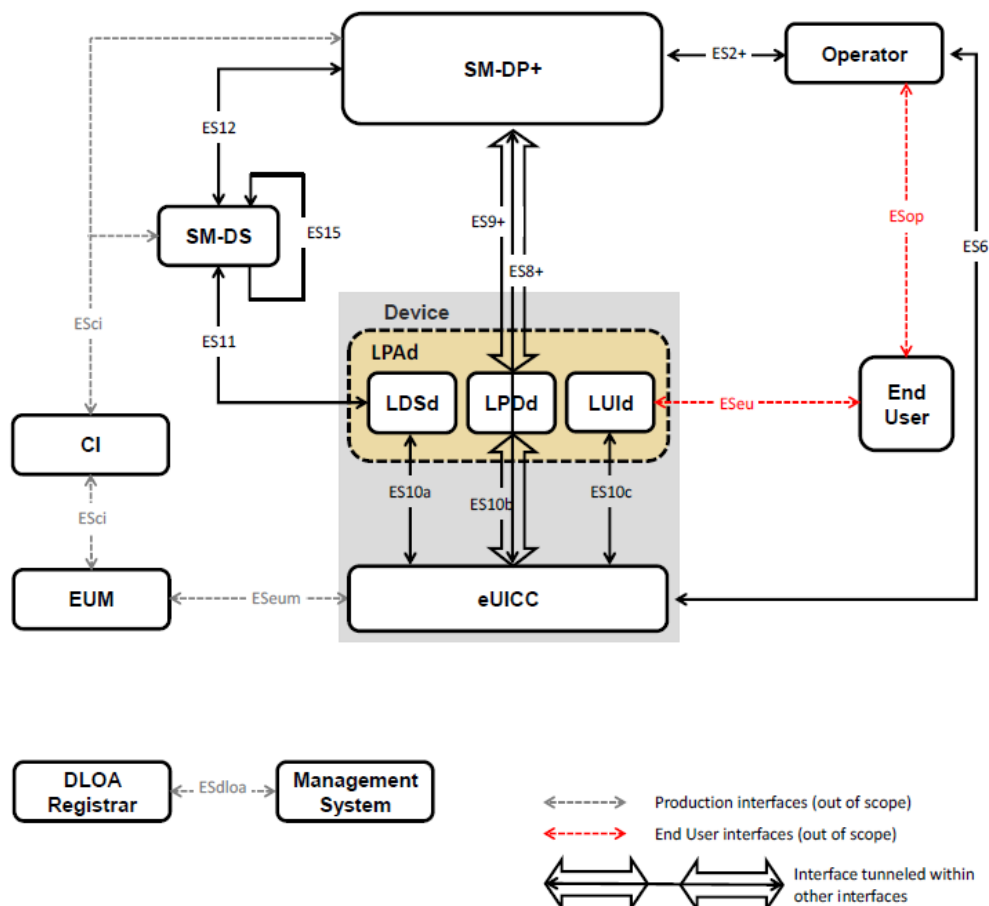
Figure 1: Remote SIM Provisioning System, LPA in the Device (Figure 1 of GSMA SGP.22 [2])
