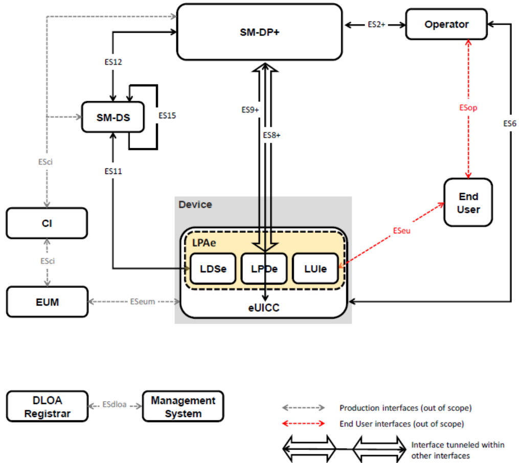
Figure 2: Remote SIM Provisioning System, LPA in the eUICC (Figure 2 of GSMA SGP.22 [2])
