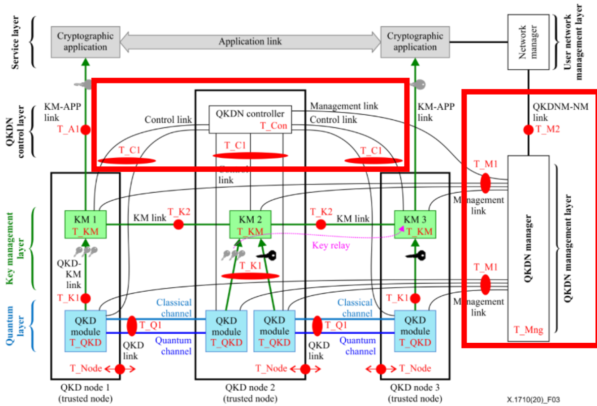
Figure 4: Security threats to the Control & Management Layer of QKDN (Ref.: ITU-T X.1710 (10/2020) )
