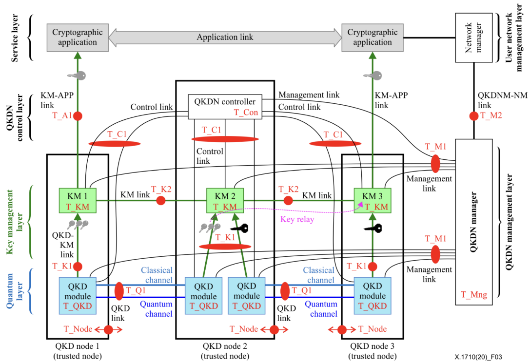
Figure 2: Security threats to QKDN (Ref.: ITU-T X.1710 (10/2020))
