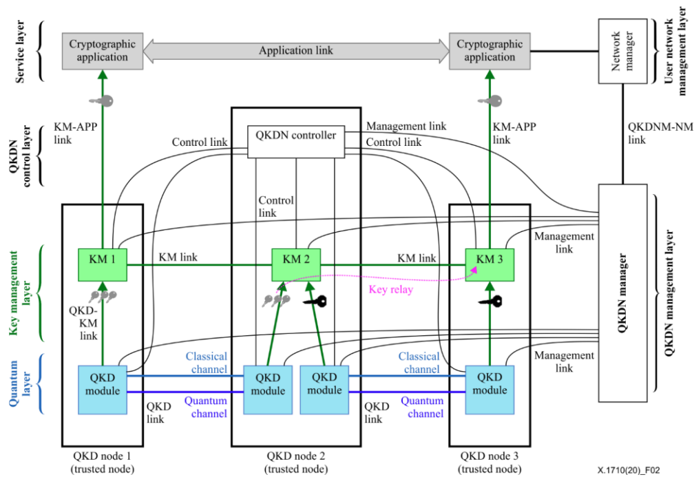
Figure 1: Typical structure of a QKDN and user network (Ref.: ITU-T X.1710 (10/2020))
