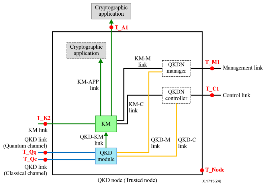
Figure 3: A typical structure of a QKD node and security threats (Ref.: ITU-T X.1713 (04/2024))
